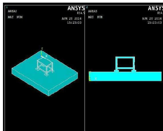
Fig-1: Isometric and front view of model 1 and model 4
