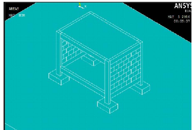
Fig -5: Isometric view of model 6
